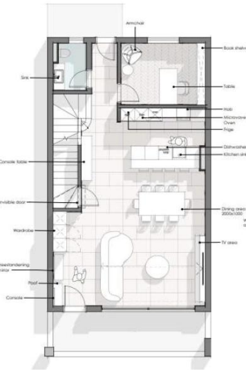
1 Furniture layout Ground floor 1:65
