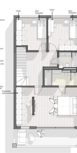
2 Furniture layout First floor 1:65
