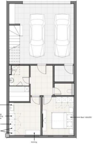
0 Furniture layout Basement floor 1:65
