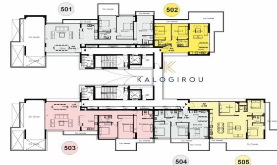
FIFTH FLOOR
