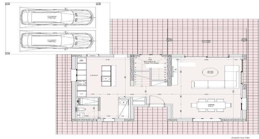
floor plans house type c ground floor
