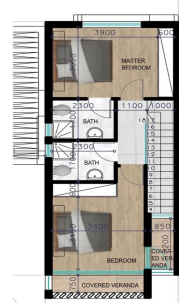
UPPER FLOOR
