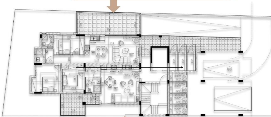
APARTMENT 001 - TWO BDR Internal Area = 75m 2 Uncovered Veranda = 27m 2
