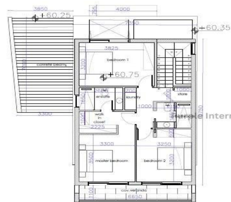
FIRST FLOOR SCALE 1:100
