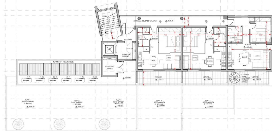
SECOND FLOOR_ LEVEL +2
