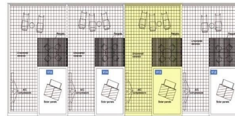
ROOF PLAN No 372/E
