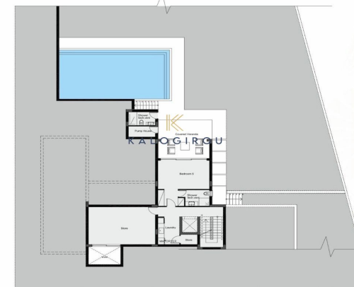
BASEMENT FLOOR
