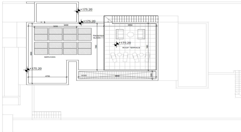
ROOF FLOOR PLAN SCALE 1:100
