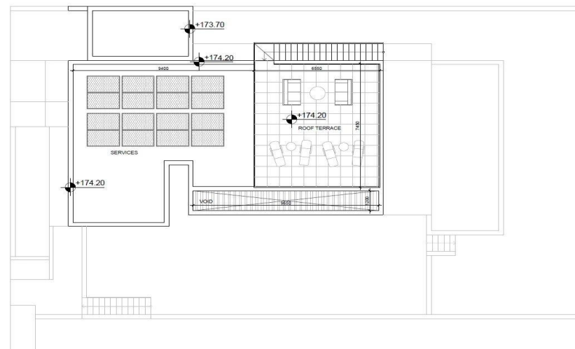
ROOF TERRACE SCALE 1:100
