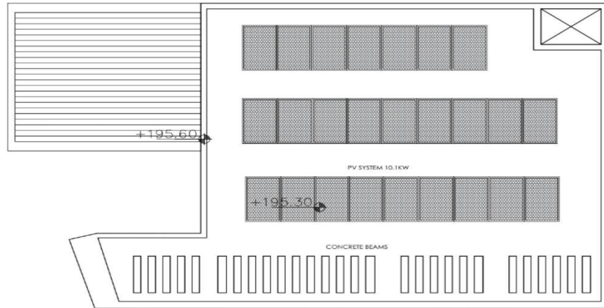
Villa 16 - Roof Plan
