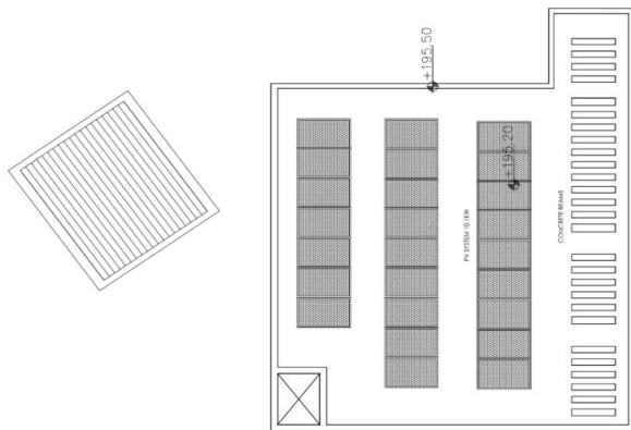
Villa 15 - Roof Plan
