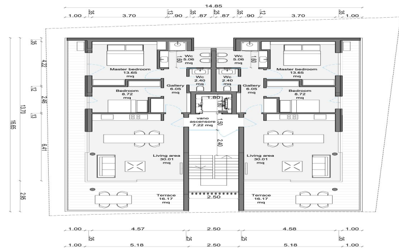
1st FLOOR Scale 1:100
