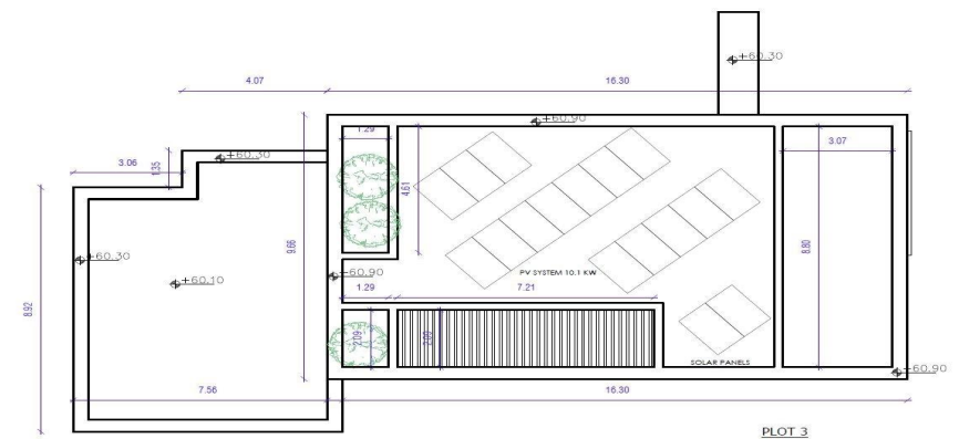
PLOT 3- GROUND FLOOR SC 1:100
