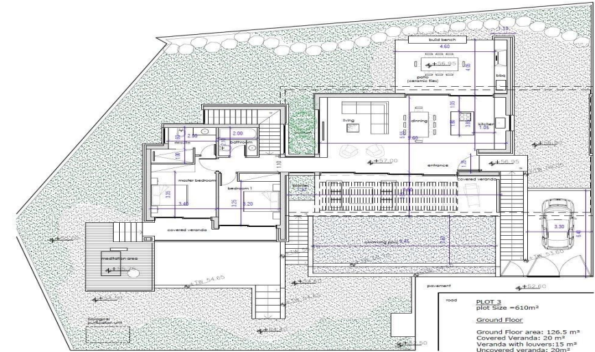
PLOT 3- GROUND FLOOR SC 1:100
