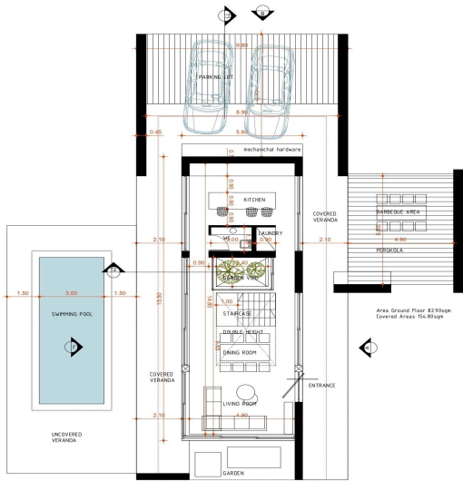
TYPE 2 | TWO STOREY ΚΑΤΩΗ ΙΣΤΙΟΦΥ
