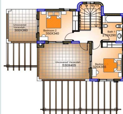
PRELIMINARY FIRST FLOOR PLAN
