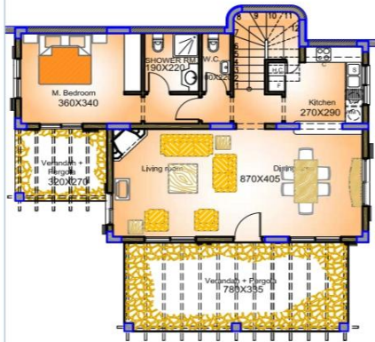
PRELIMINARY GROUND FLOOR PLAN
