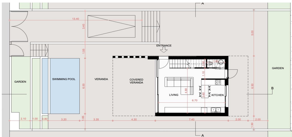
HOUSE TYPE C- HOUSES 17-22 TWO STOREY HOUSE WITH ROOF GARDEN
