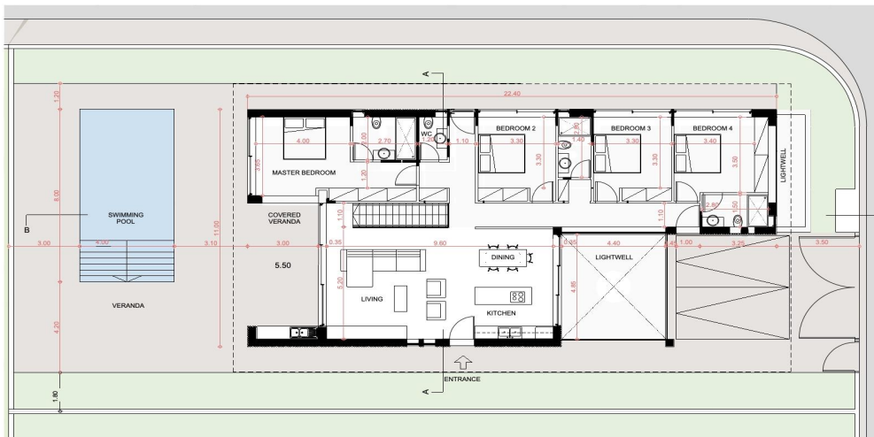
HOUSE TYPE A- HOUSES 01-04 SINGLE STOREY HOUSE WITH BASEMENT
