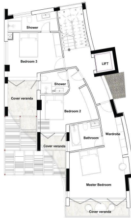
Villa 2 - First Floor Plan
