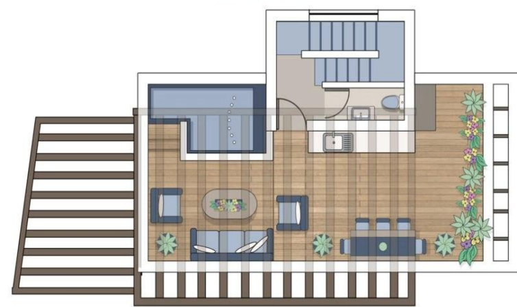
Roof Garden Plan
