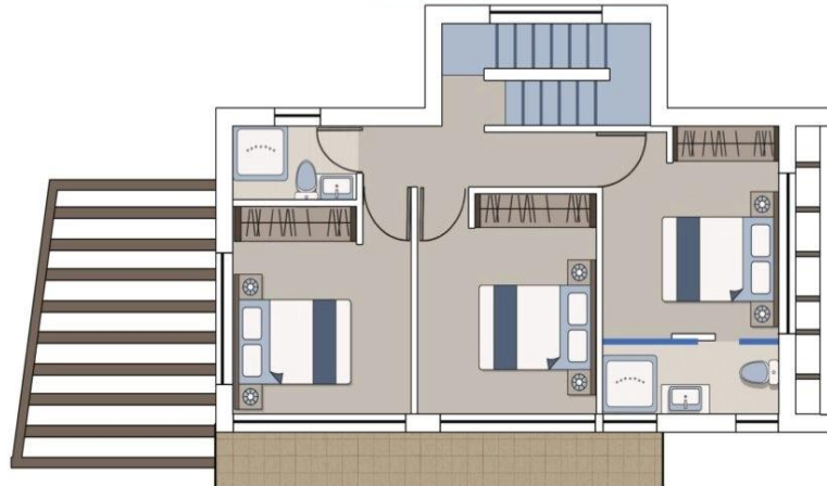
Firsst Floor Plan
