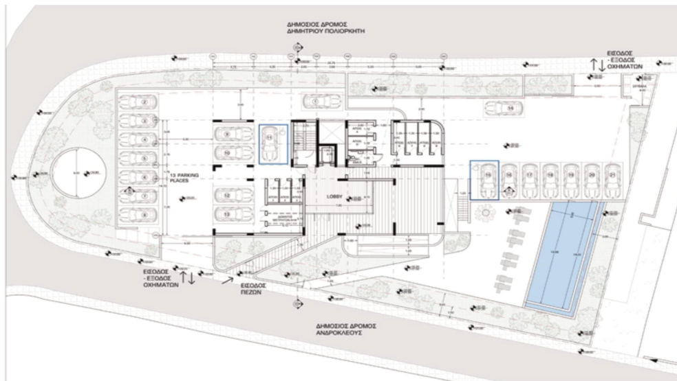
Ground Floor: 13 Parking Spaces | Lobby entrance | Swimming Pool Access
