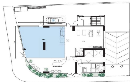
GROUND FLOOR PLAN SCALE 1:100
