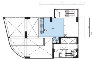
MIDDLE FLOOR PLAN SCALE 1:100
