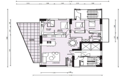
2nd-3rd FLOOR PLAN SCALE 1:100
