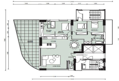
1st FLOOR PLAN SCALE 1:100
