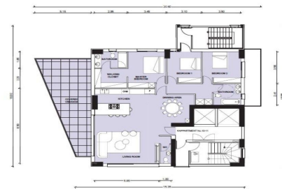
10th-11th FLOOR PLAN SCALE 1:100
