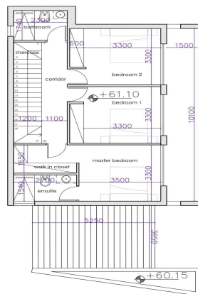
FIRST FLOOR SCALE 1:100
