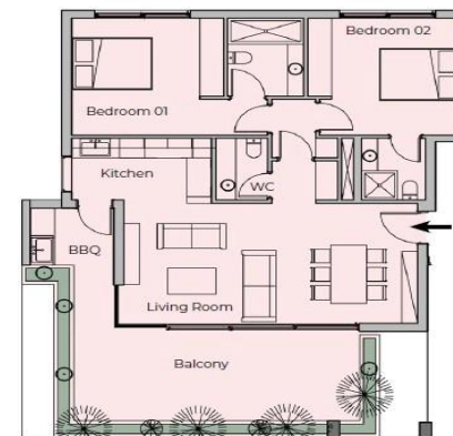
APARTMENTS 101 - 201 - 301
