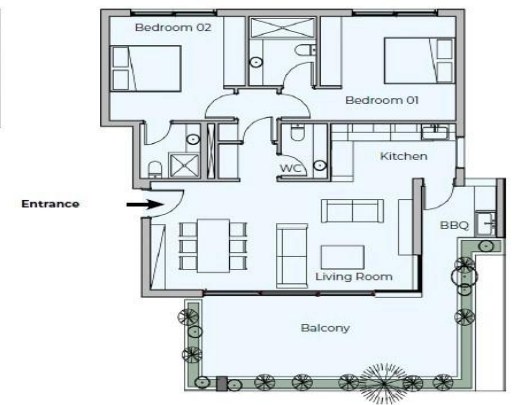
APARTMENTS 102 - 202 - 302
