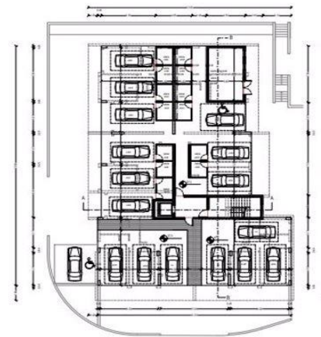
ground floor plan Block A
