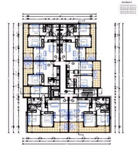
1st floor plan Block A
