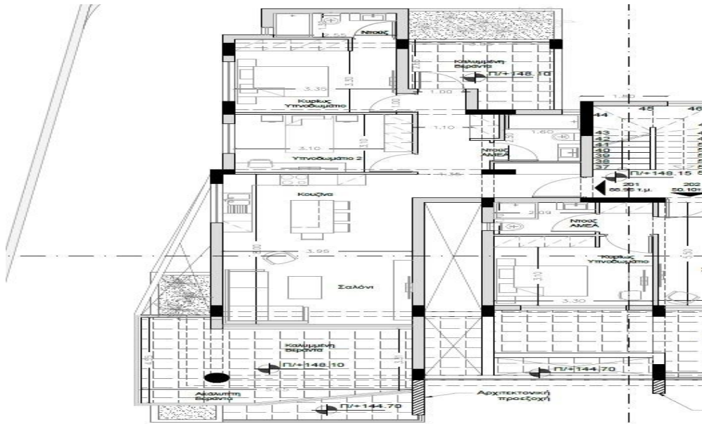
First Level
