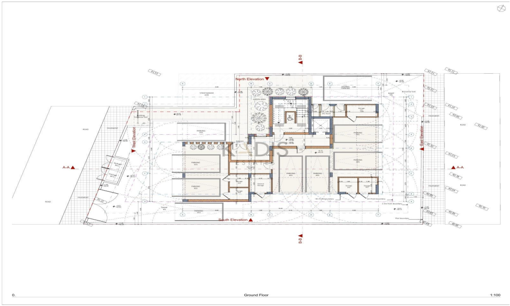
Ground Floor 1:100
