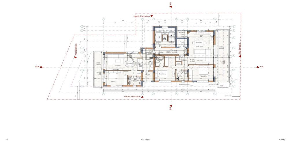
1st Floor 1:100
