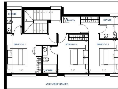
2 FIRST FLOOR 1 : 100
