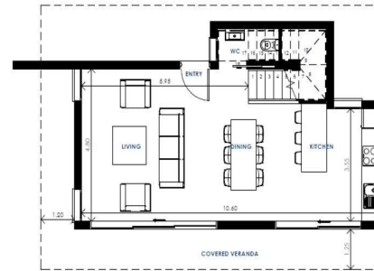
1 GROUND FLOOR 1:100
