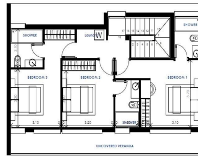
2 FIRST FLOOR 1 : 100
