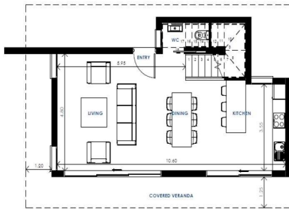
1 GROUND FLOOR 1 : 100
