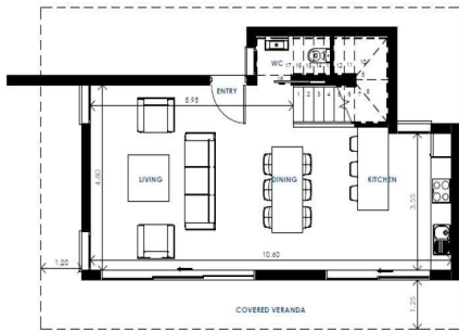
1 GROUND FLOOR 1 : 100
