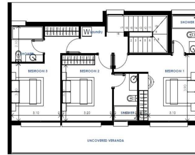
2 FIRST FLOOR 1 : 100
