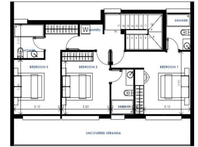
2 FIRST FLOOR 1:100
