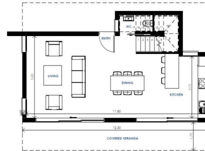
1 GROUND FLOOR 1 : 100
