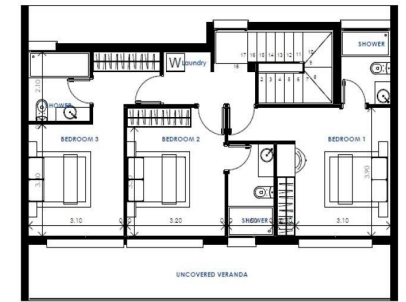
2 FIRST FLOOR 1 : 100
