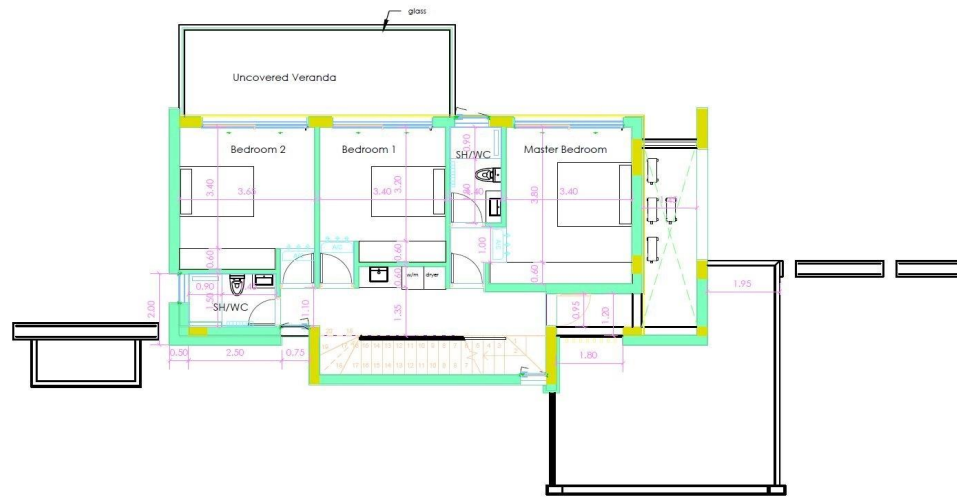
First Floor - House06
