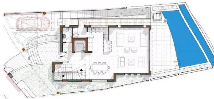
PRELIMINARY GROUND FLOOR
