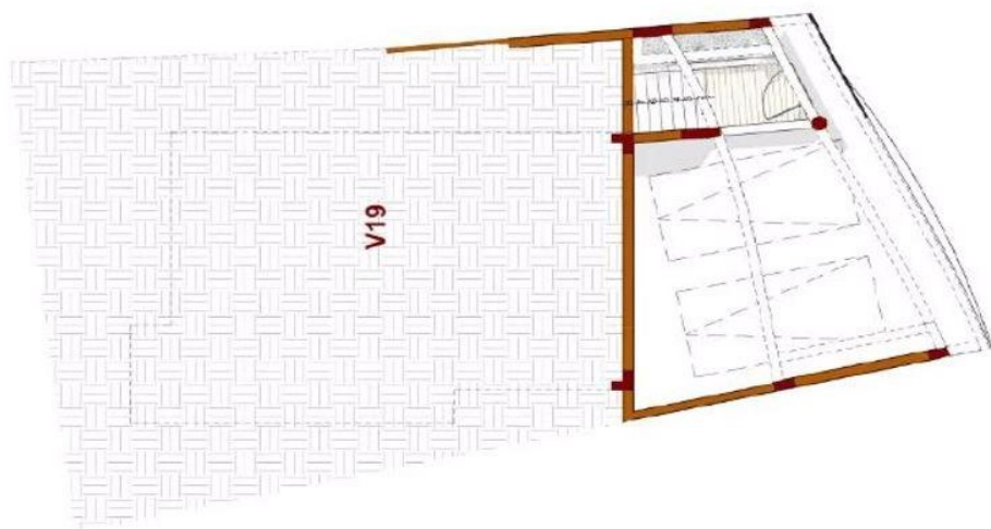
PRELIMINARY LOWER GROUND FLOOR 1
