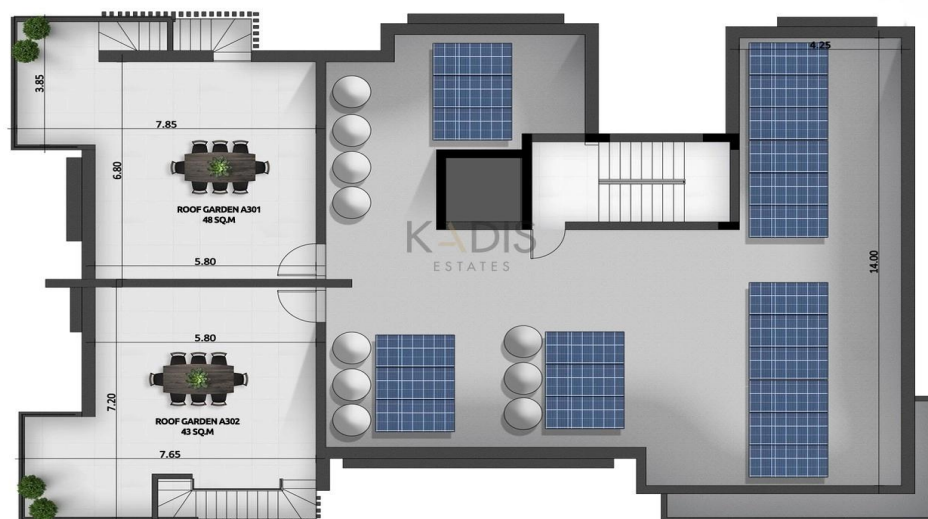
Floor Plan Roof
