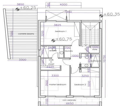
FIRST FLOOR SCALE 1:100
