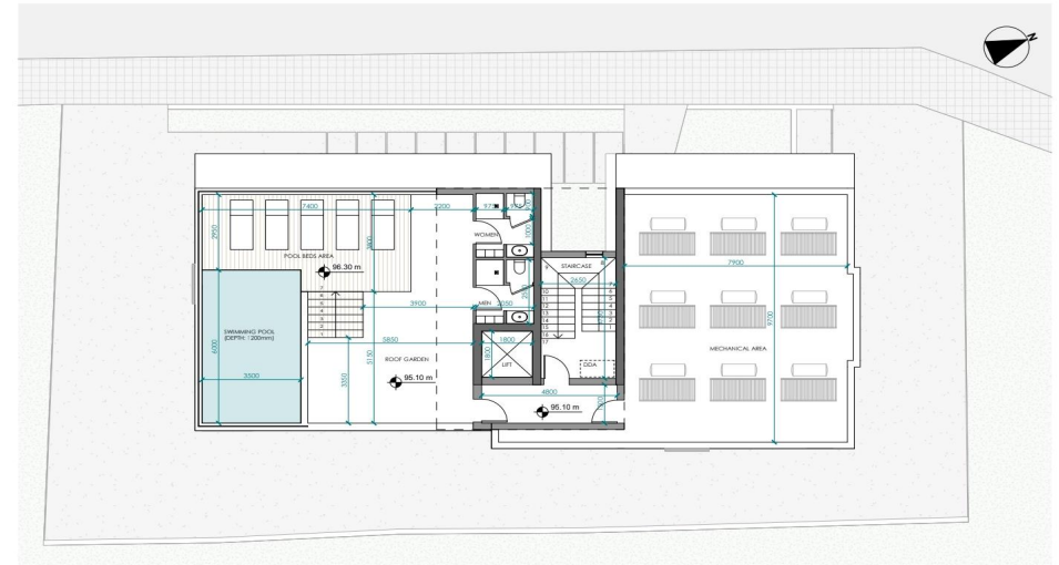
ROOF PLAN 1:100
