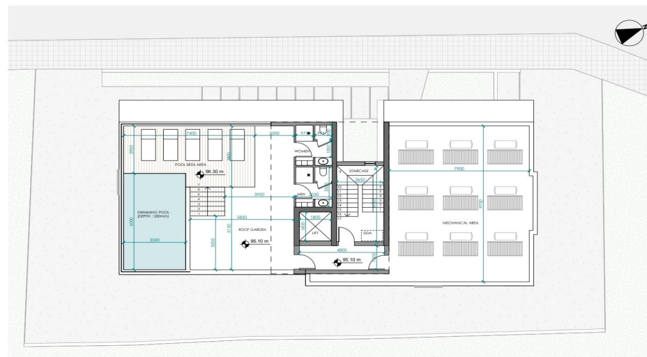
ROOF PLAN 1:100
