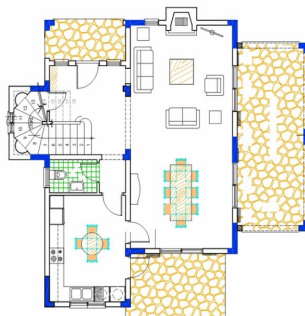
PRELIMINARY GROUND FLOOR
