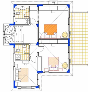
PRELIMINARY FIRST FLOOR
