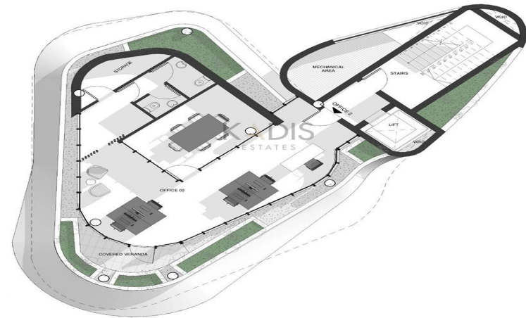
Second Floor | Offices
