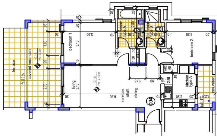
APARTMENT PLAN
