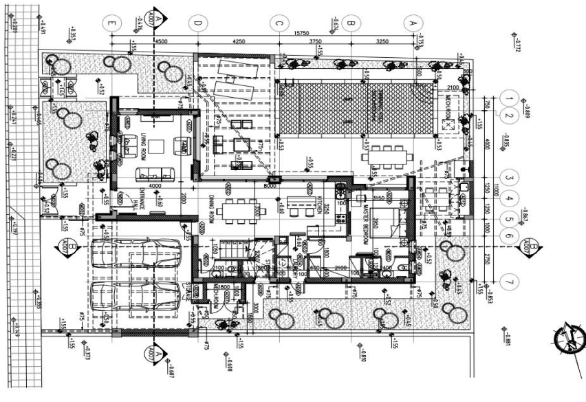
HOUSE CAMELIA - GROUND FLOOR PLAN
