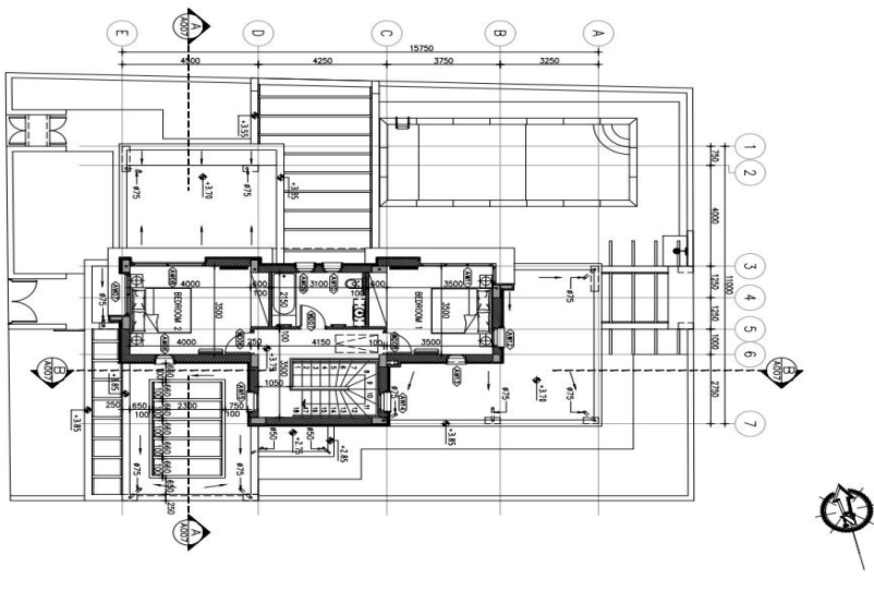
HOUSE CAMELIA - FIRST FLOOR PLAN
