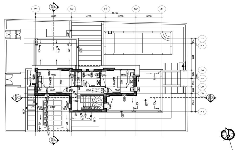
HOUSE CAMELIA – FIRST FLOOR PLAN
