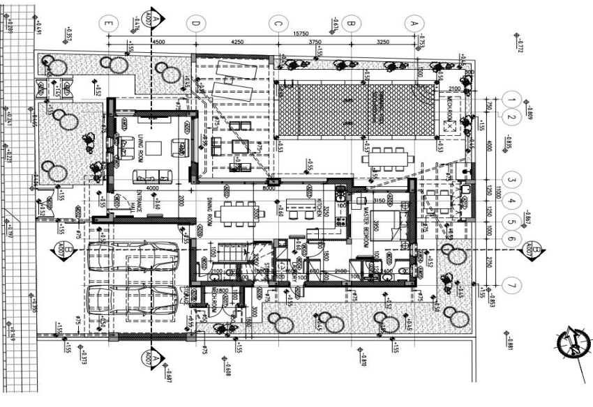
HOUSE CAMELIA – FIRST FLOOR PLAN SCALE 1:100
