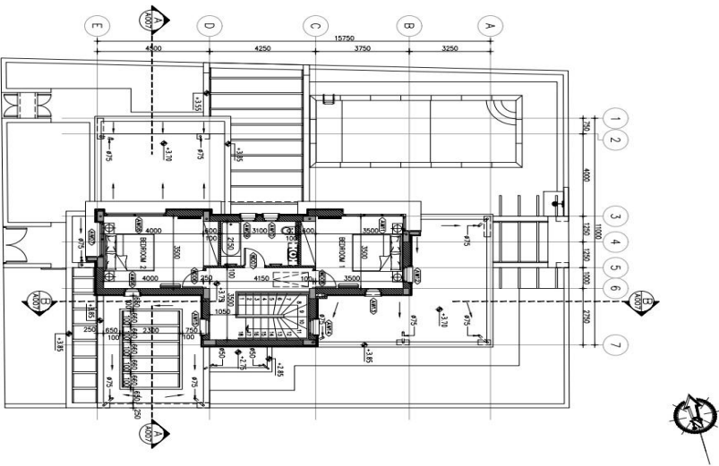
HOUSE CAMELIA – FIRST FLOOR PLAN SCALE 1:100
