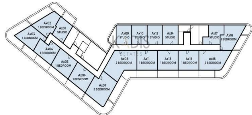
Indicative Residential Floor Plans Building A (2 nd , 3 rd , 4 th floor)
