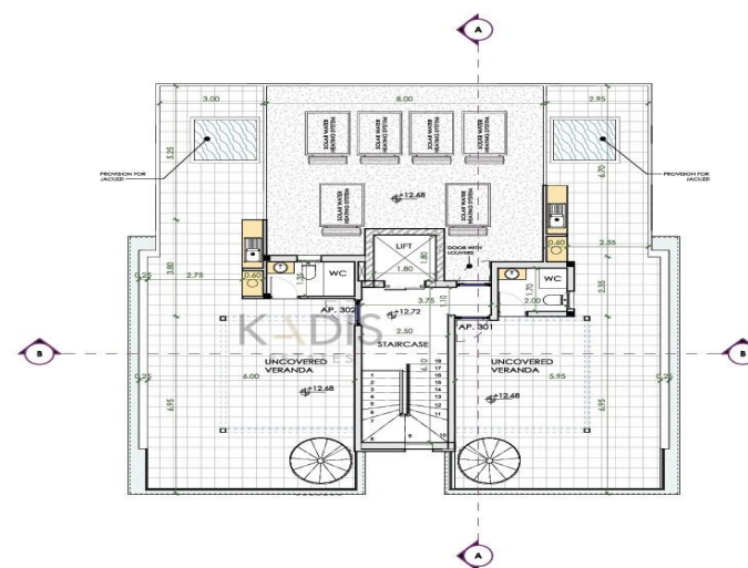
ROOF GARDEN FLOOR PLAN
