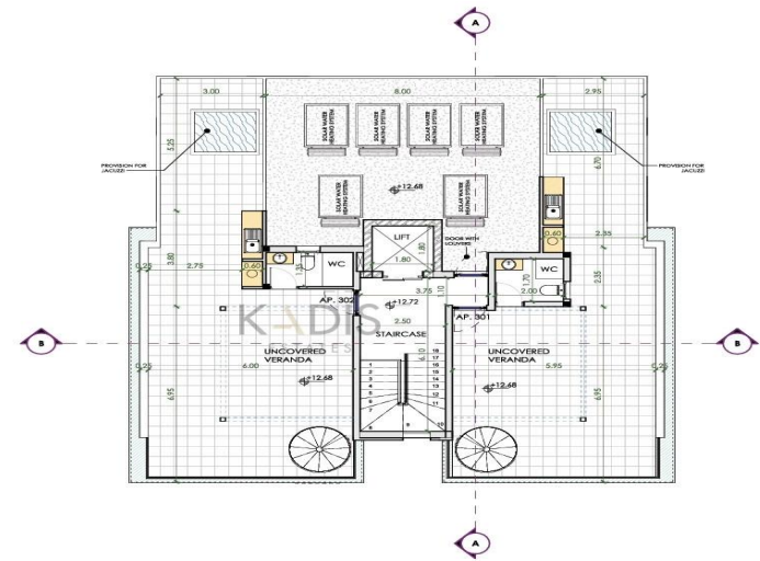
ROOF GARDEN FLOOR PLAN
