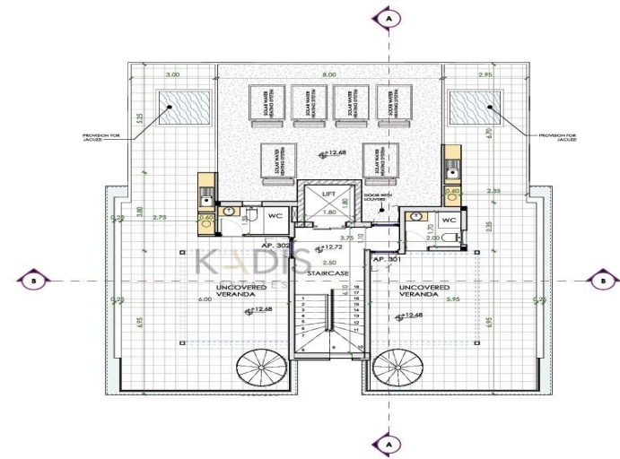
ROOF GARDEN FLOOR PLAN
